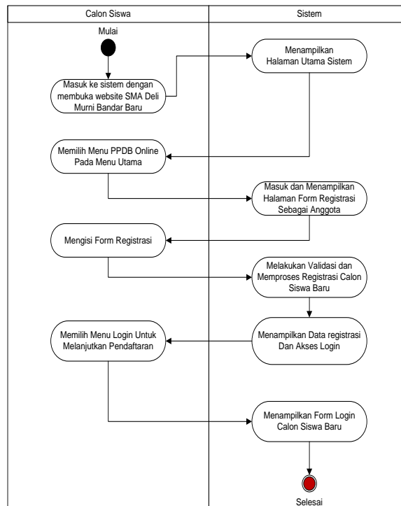
Gambar 2. Diagram activity proses registrasi
